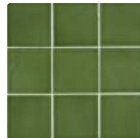
Lichen
